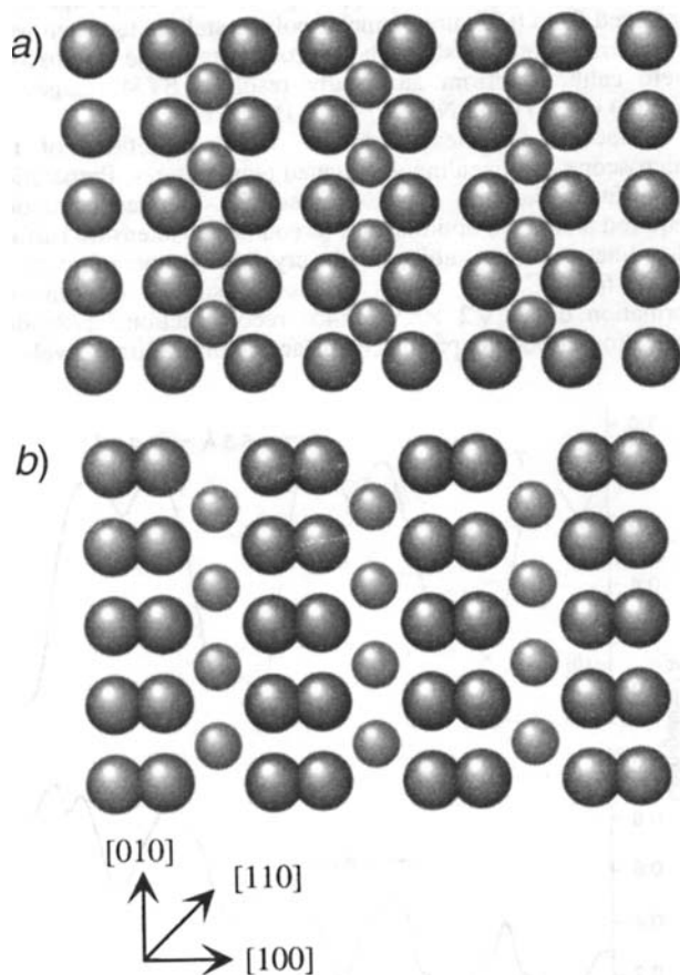
Fig. 3 Schematic representation of \text{Na}_{0.5}\text{O} plane on \text{Na}_{0.5}\text{WO}_3(001) . The ions are assigned the ionic radii tabulated by Shannon and Prewitt. Large ions are \text{O}^{2-} ; small ions are \text{Na}^+ . (a) Unrelaxed structure derived from bulk lattice parameter. (b) Relaxed surface structure deduced from STM image. The \text{O}^{2-} ions are seen to overlap.
